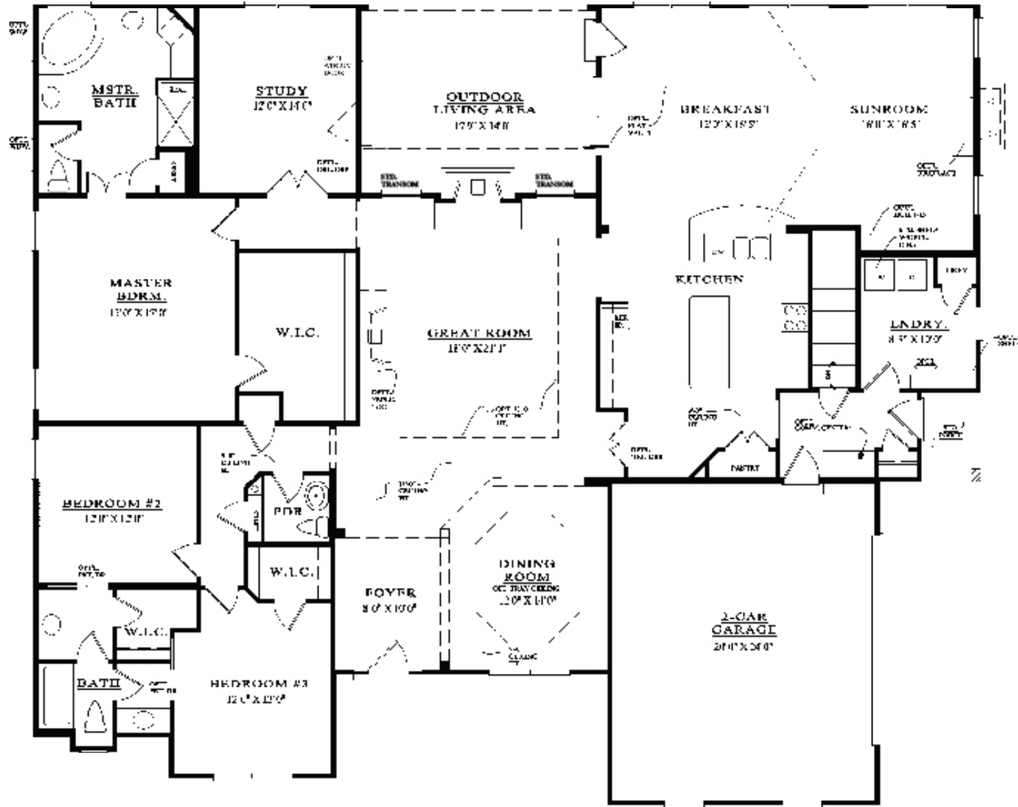
Floor Plan
