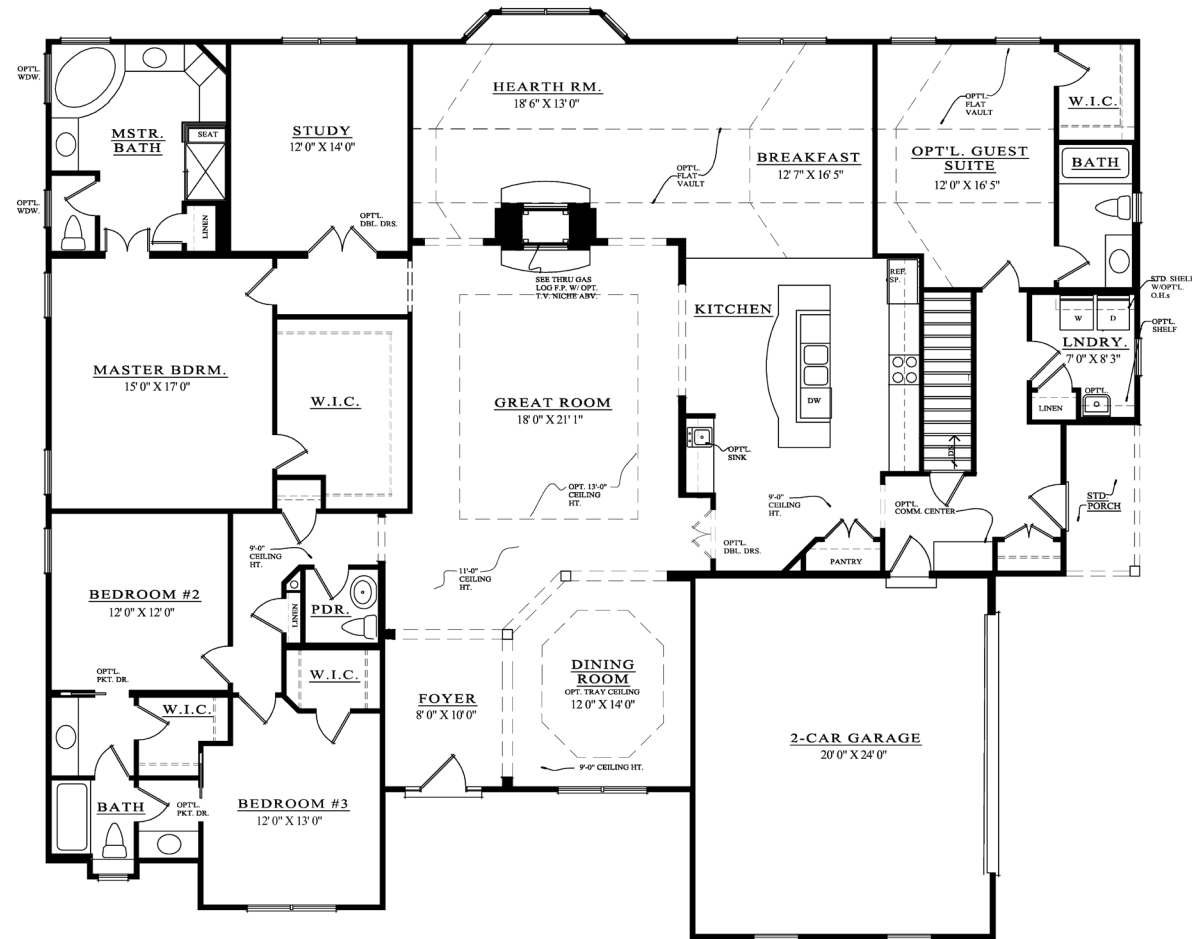
Floor Plan with Optional Guest Suite and Hearth Room
